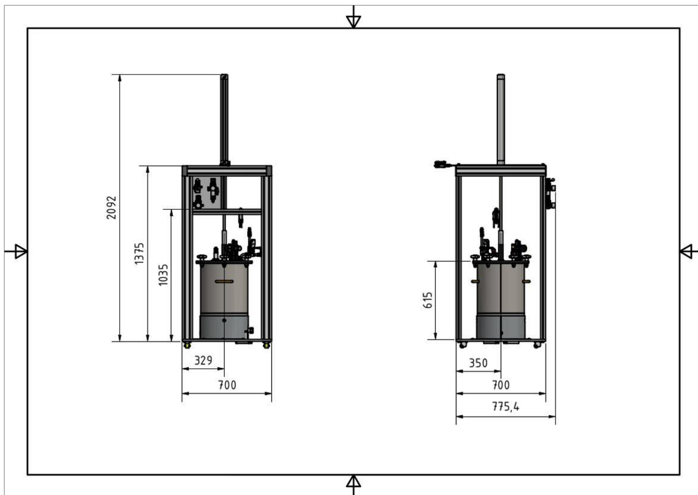
Dimensional drawing (Dimensions in mm)
