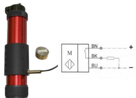
9020 Magnetic limit sensor
